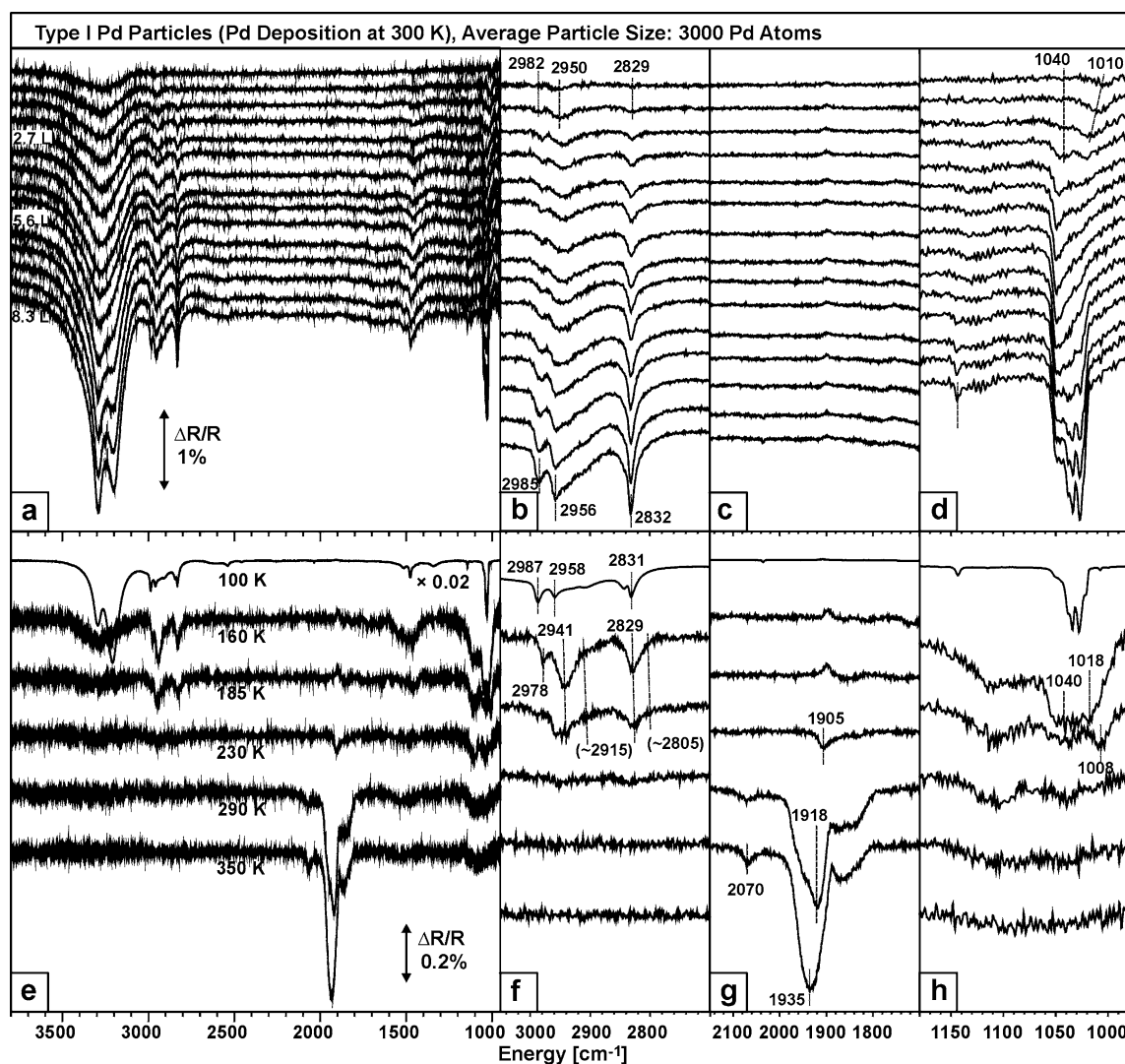
Fig. 5. IR reflection absorption spectra recorded during methanol adsorption at 100 K (a–d) and during methanol decomposition at various temperatures (e–h) on a Pd model catalyst of type I. The spectra e–f were recorded during exposure to a molecular beam of methanol (in Ar as a carrier gas, see text for details).
