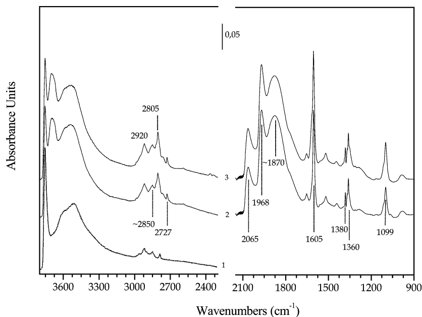
Fig. 4. FTIR spectra of CO/H 2 mixture (1/2) adsorbed on Pd/MgO outgassed and reduced at 623 K: exposure at 423 K for 15 min (curve 2) and at 473 K for 15 min (curve 3). Curve 1 reports the spectrum before CO/H 2 mixture adsorption.
