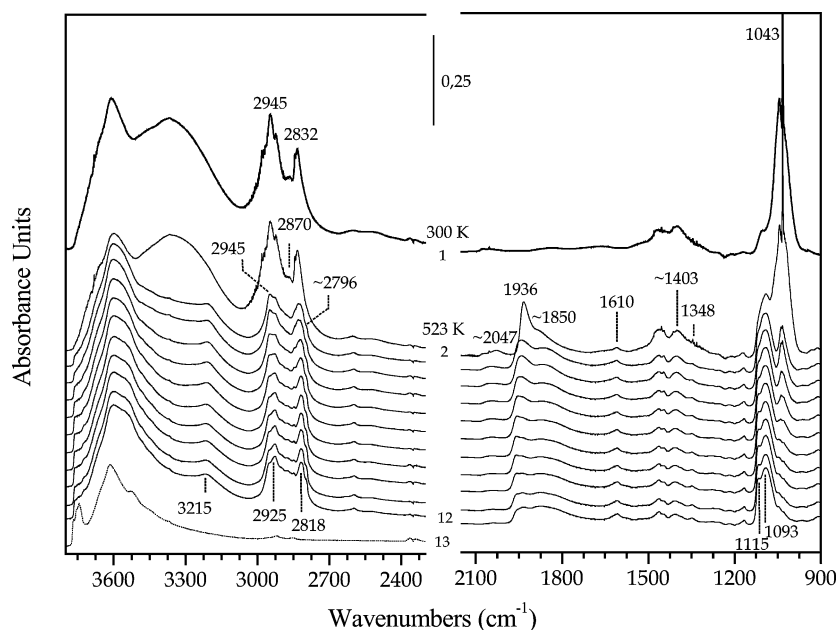
Fig. 2. FTIR spectra of \text{CH}_3\text{OH} adsorbed on \text{PdMgO}(\text{Cl}) outgassed and reduced at 623 K. Curve 1 shows the spectrum of \text{CH}_3\text{OH} dosed at 300 K ( p = 2.66 kPa); curve 2 shows the spectrum after thermal treatment in \text{CH}_3\text{OH} at 523 K; curve 12 shows the spectrum after thermal treatment in \text{CH}_3\text{OH} at 523 K and at \theta(\text{CH}_3\text{OH}) \rightarrow 0 ; curve 13 shows the spectrum before \text{CH}_3\text{OH} adsorption.
