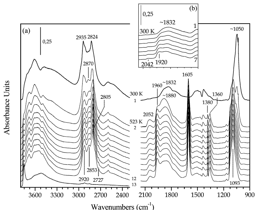
Fig. 3. FTIR spectra of \text{CH}_3\text{OH} adsorbed on Pd/MgO outgassed and reduced at 623 K. (a) Curve 1 shows the spectrum of \text{CH}_3\text{OH} dosed at 300 K ( p = 2.66 kPa); curve 2 shows the spectrum after thermal treatment in \text{CH}_3\text{OH} at 523 K; curve 12 shows the spectrum after thermal treatment in \text{CH}_3\text{OH} at 523 K and at \theta(\text{CH}_3\text{OH}) \rightarrow 0 ; curve 13 shows the spectrum before \text{CH}_3\text{OH} adsorption. (b) FTIR spectra in the CO stretching region of \text{CH}_3\text{OH} adsorbed at 300 K on Pd/MgO outgassed and reduced at 623 K (curve 1 shows the spectrum at p(\text{CH}_3\text{OH}) = 2.66 kPa; curve 7 shows the spectrum at p(\text{CH}_3\text{OH}) \cong 2 Pa).
